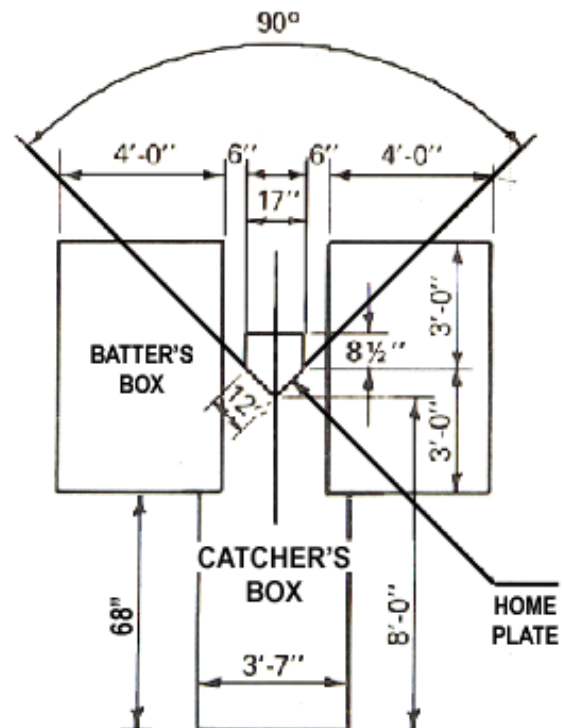
Regulation Baseball Home Plate Layout
